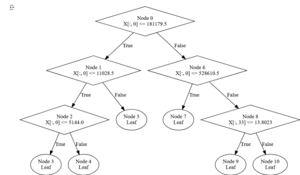
Figure 1. Decision Tree of new approach used for intrusion detection
