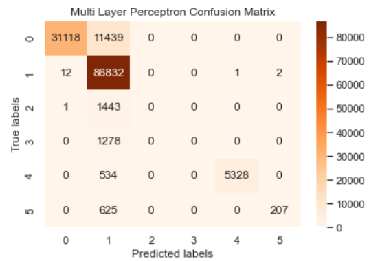
Figure 6. Confusion Matrix of Multi-Layer Perceptron Classifier
