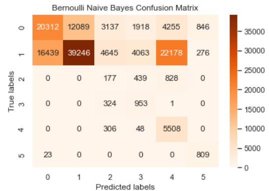
Figure 7. Confusion Matrix of Bernoulli naive bayes classifier
