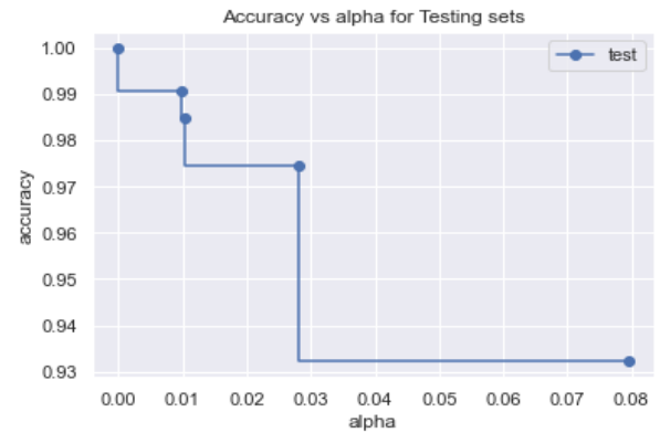
Figure 4. The relationship between the effective alpha parameter and the accuracy of the decision tree model on the test data
