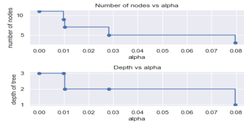
Figure 3. Relationship between Effective Alpha and number of nodes
