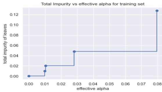
Figure 2. Correlation between the total impurity and the effective alpha parameter
